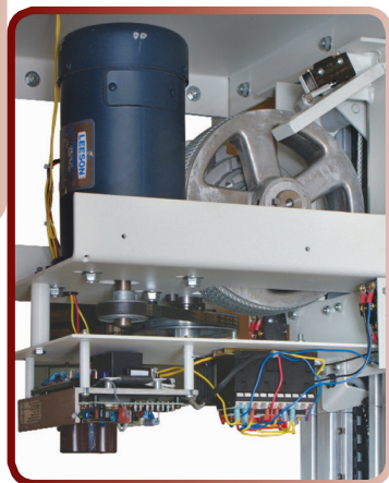
Electric motor, cable-drum drive system and limit switches are pre-installed under the car.
